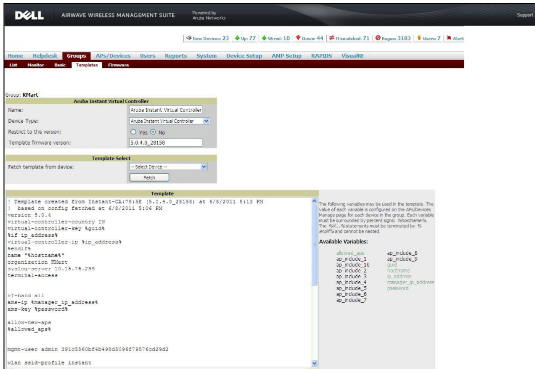
Figure 95 Template-based Configuration
